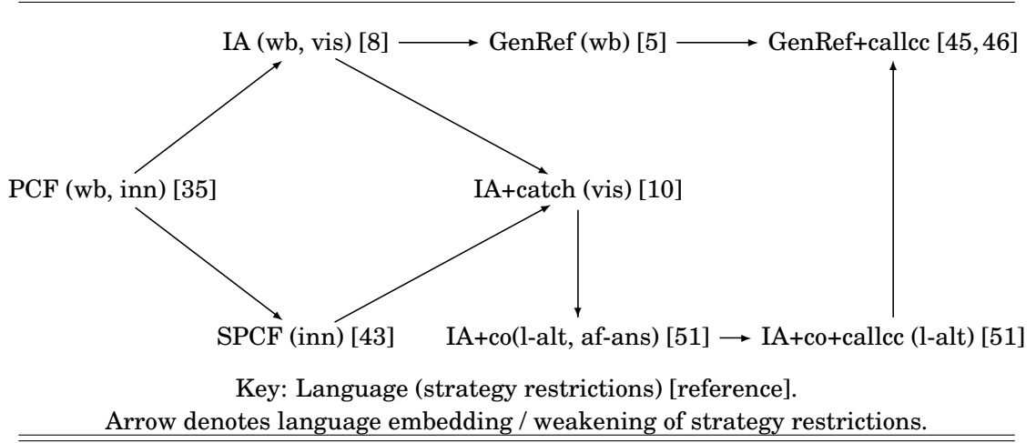
Figure 1-1: Programming Languages and Hyland-Ong Games Models
